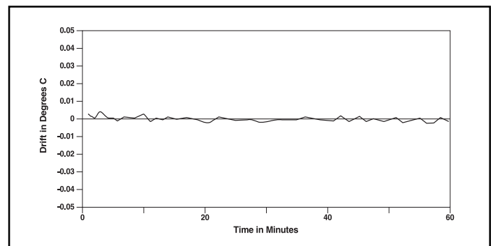
Figure 2. LDT-5412 Short-Term Stability Measurement Results.
